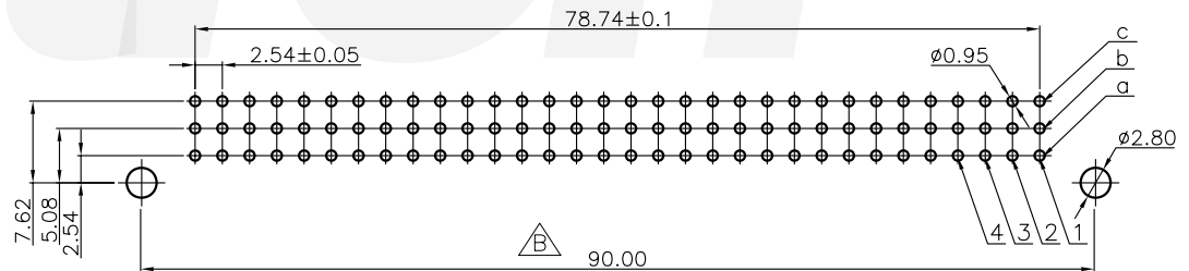
PCB Layout
